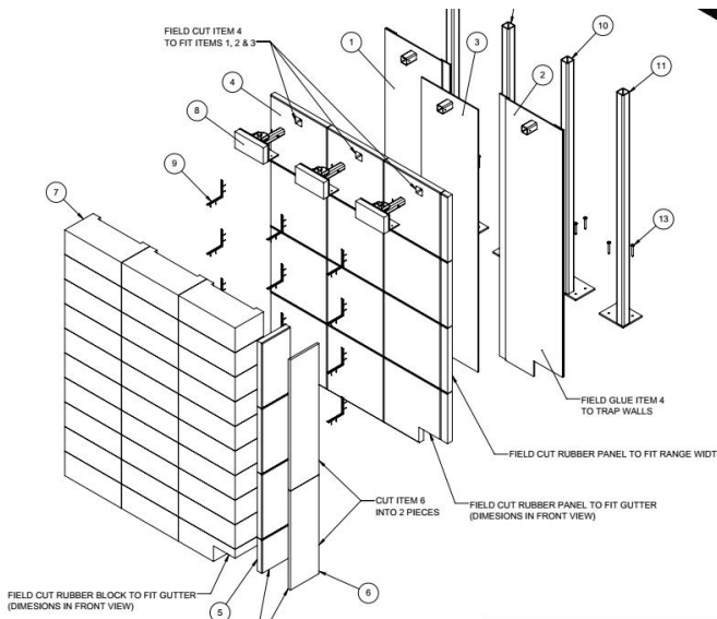
Freestanding Installation
